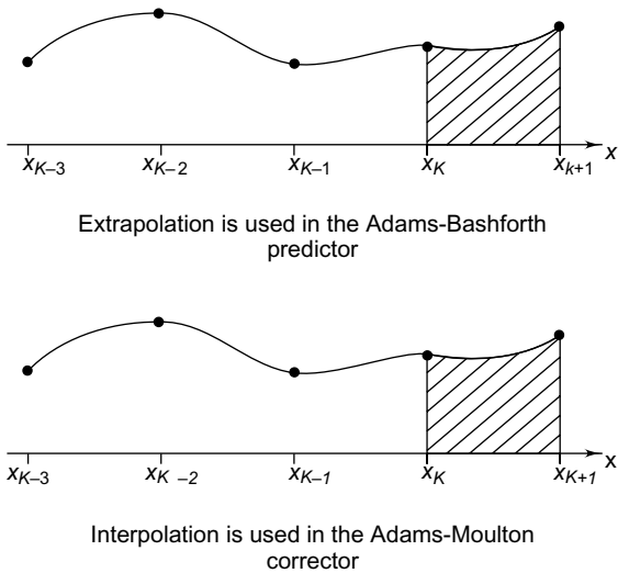
Fig. 33.2 Integration on the interval x_k, x_{k+1}
