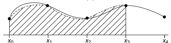
Simpson's \frac{3}{8} rule on [x_0, x_3]
