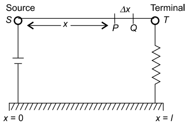
Fig. 19.21 Transmission line
