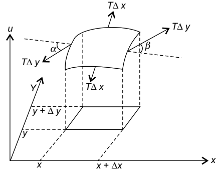
Fig.19.17 Vibrating membrane
